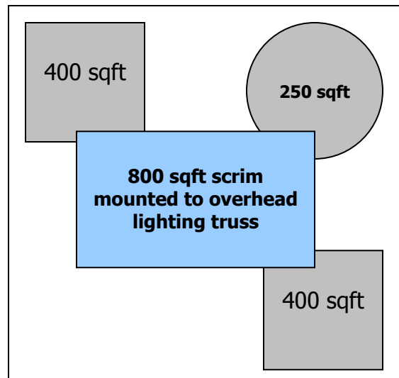
The addition of the lighting scrim results in the entire booth being classified as one covered area (exceeding 750 sqft). ALL covered elements must be protected by an AFSS.
